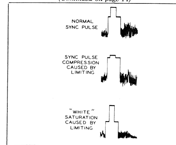
Figure 5. Sync-pulse compression
