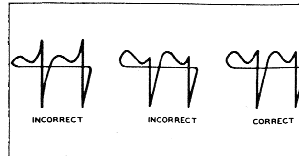
Figure 11. Horizontal-oscillator waveforms
