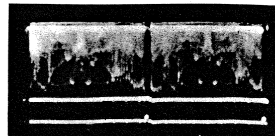
Figure 4. Vertical-sync pulse in composite signal
