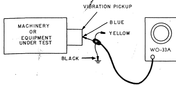
Figure 19. Vibration analysis setup
