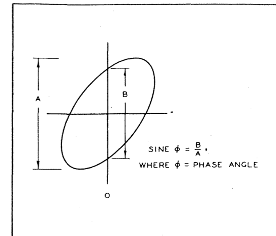
Figure 16. Measurement of phase shift
