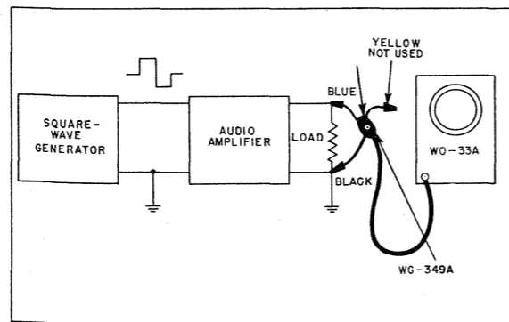
Figure 14. Audio amplifier test setup
