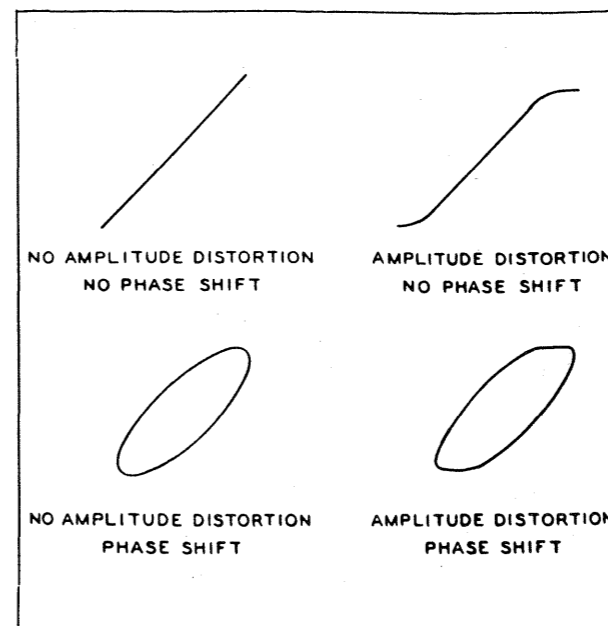
Figure 15. Distortion and phase shift in audio amplifier
