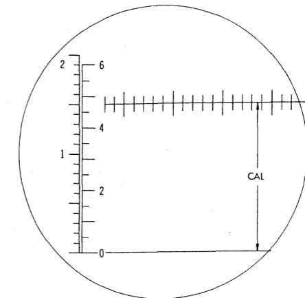
Figure 2. WO-33A graph screen with voltage scales
