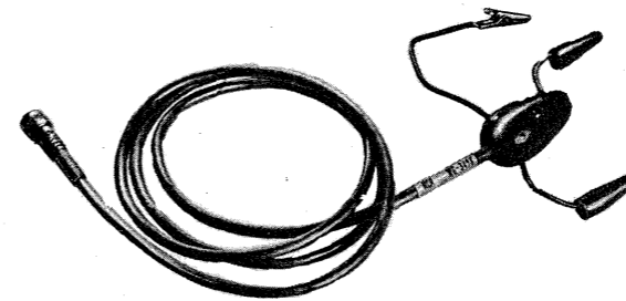
Figure 1. WG-349A direct/low-capacitance probe and cable supplied with WO-33A
