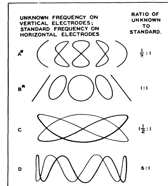
Figure 17. Lissajous figures
