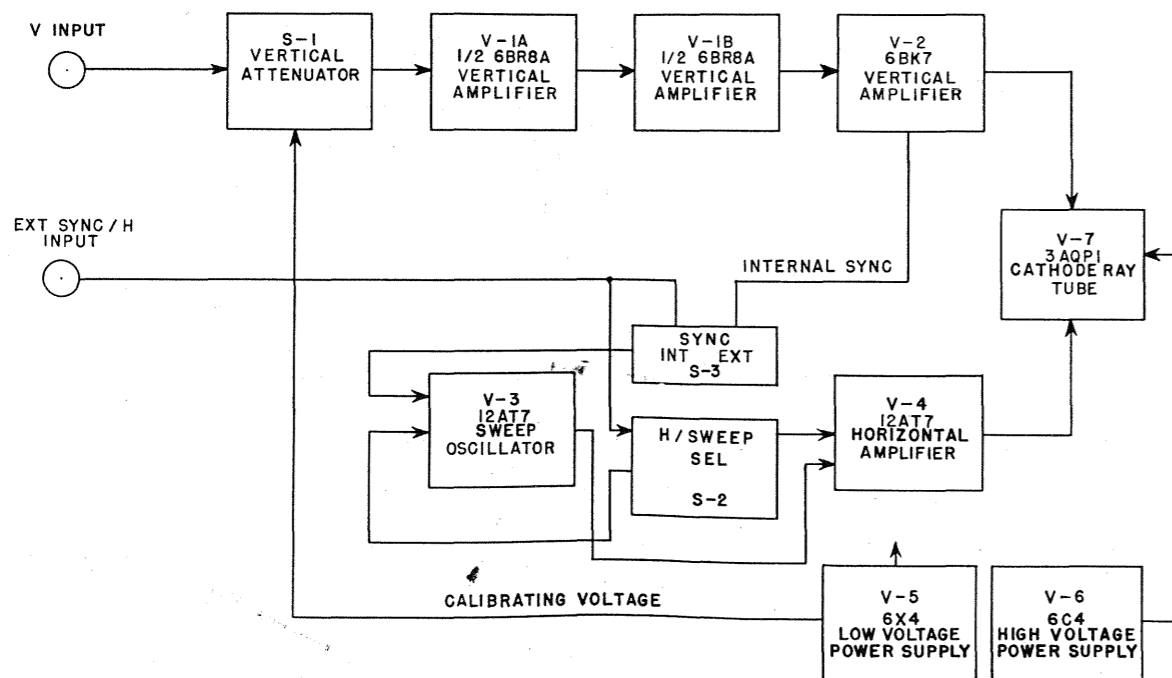
Figure 20. Block Diagram WO-33A
