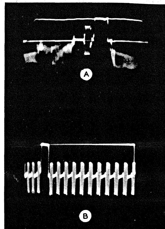
Figure 13. Color-TV signals as displayed by WO-33A. (A) Composite color-TV signal. Color-burst can be seen to left of sync pulse. (B) Output signal from RCA WR-61A Color-Bar Generator showing color-sync pulses and 10 color-bar pulses.
